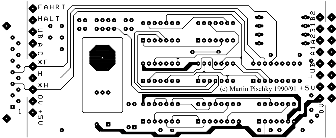
LAYOUT TOP-SIDE
