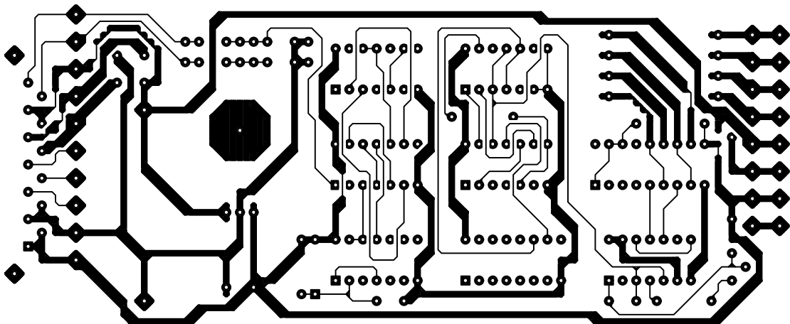
LAYOUT BOTTOM-SIDE
