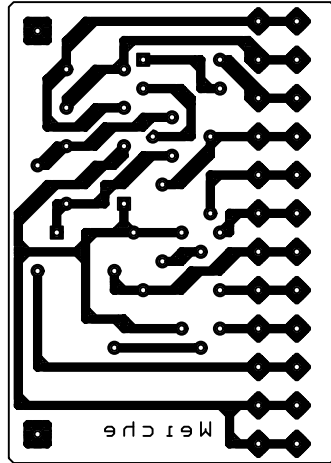
LAYOUT BOTTOM-SIDE
