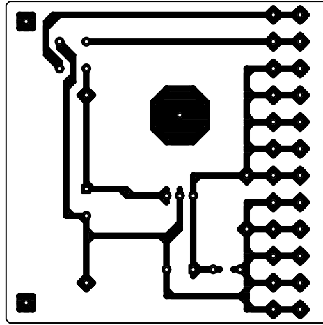
LAYOUT BOTTOM-SIDE
